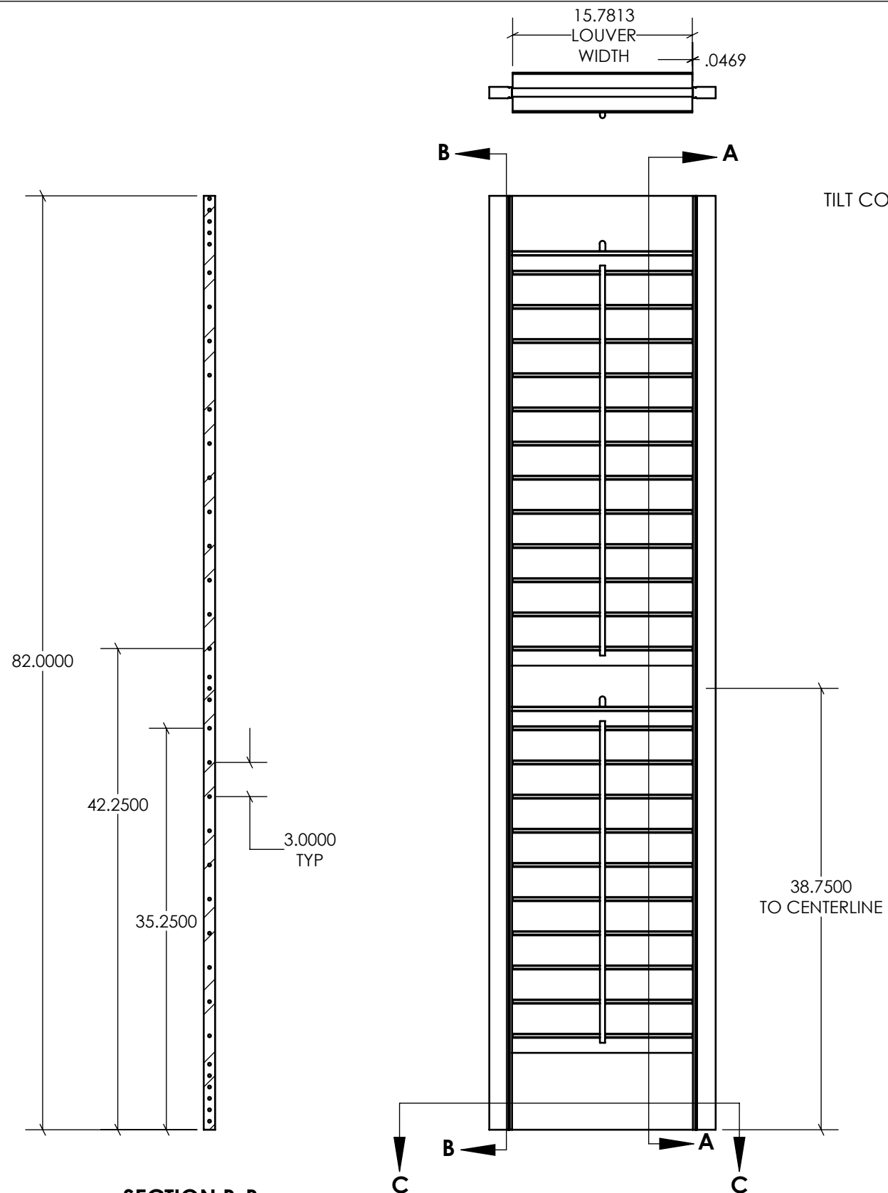
SECTION B-B (LOUVER HOLE LOCATIONS)
