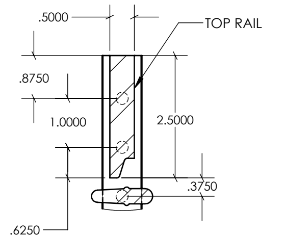
DETAIL H
