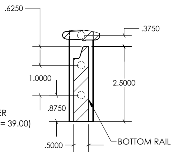
DETAIL J
