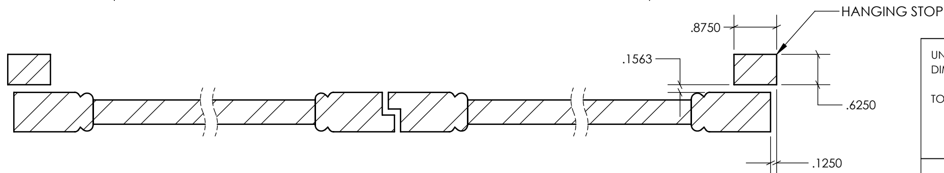
SECTION B-B
