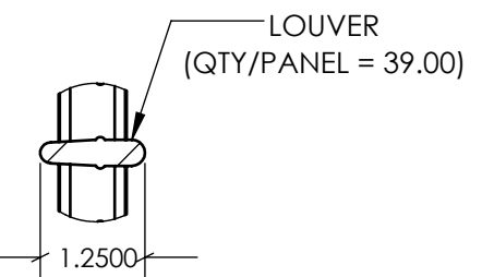
DETAIL J
